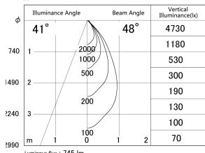
Direct Horizontal Illuminance DD146-0850DW9035
