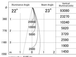
Direct Horizontal Illuminance DD146-4025DW9035
