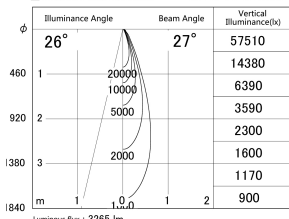
Direct Horizontal Illuminance DD146-3025DB9035
