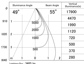
■ Direct Horizontal Illuminance DD146-4050DB9035
