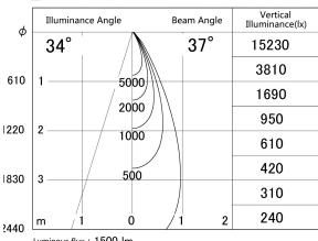
■ Direct Horizontal Illuminance DD146-1535DW9040
