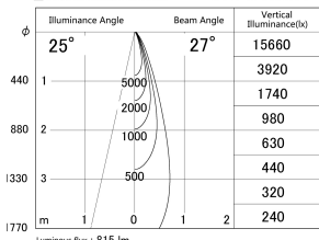
■ Direct Horizontal Illuminance DD146-0825WW9027
