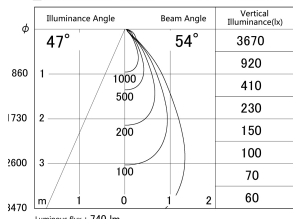
Direct Horizontal Illuminance DD146-0850WW9027
