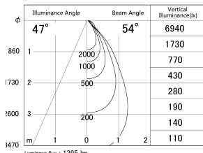
■ Direct Horizontal Illuminance DD146-1550WW9027
