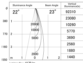
Direct Horizontal Illuminance DD146-4025WW9027
