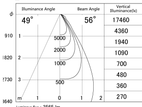
Direct Horizontal Illuminance DD146-4050WW9027
