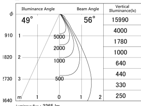
Direct Horizontal Illuminance DD146-3550WW9030
