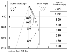
■ Direct Horizontal Illuminance DD146-0835WW9035
