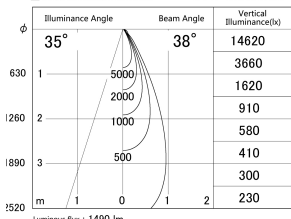
Direct Horizontal Illuminance DD146-1535WW9035
