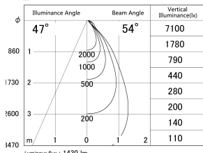
■ Direct Horizontal Illuminance DD146-1550WW9040
