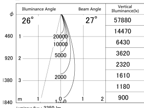
Direct Horizontal Illuminance DD146-3025WW9040
