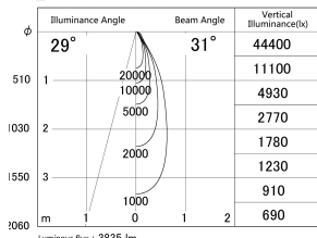
Direct Horizontal Illuminance DD146-3535WW9040
